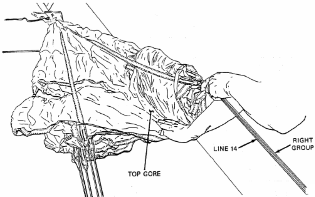
Figure 10. Flipping Right Gore Group.
