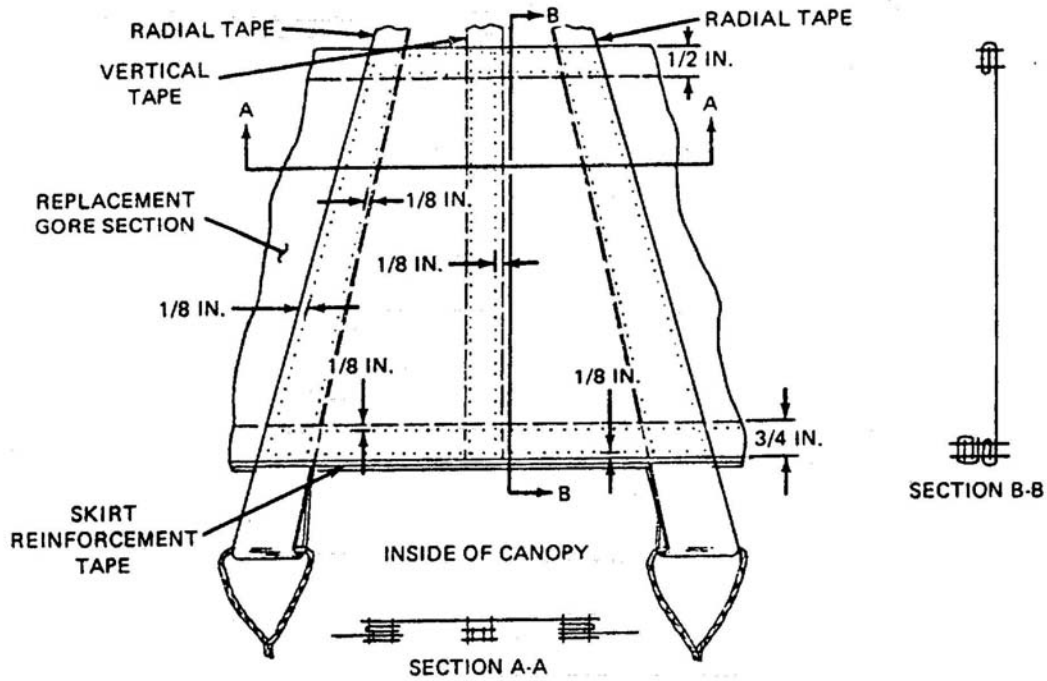
Figure 3. Gore Section 1, Replacement Details.
