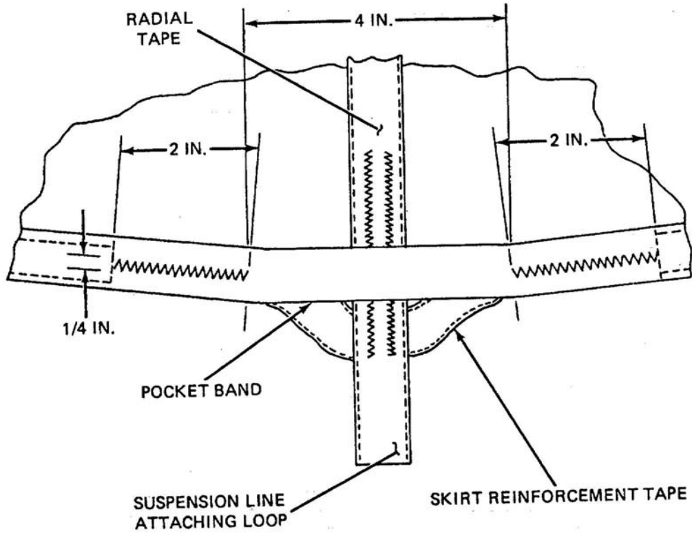
Figure 1. Pocket Band Replacement Details.
