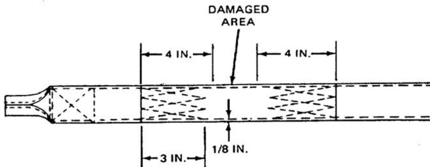
Figure 2. Riser Splicing Details.
