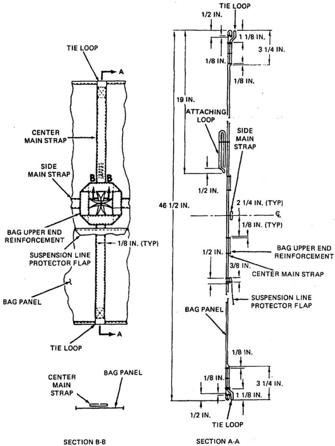
Figure 3. Center Main Strap Installation Details.
