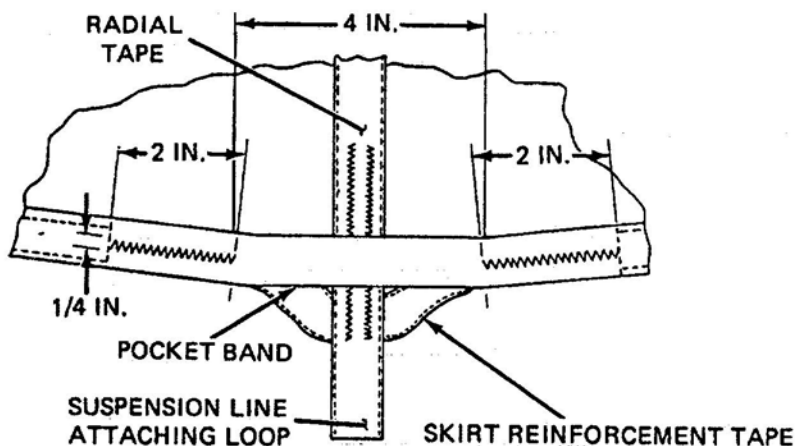
Figure 4. Reinstalling Pocket Band.
