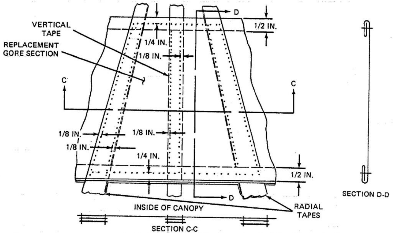
Figure 5. Gore Section 2, Replacement Details.
