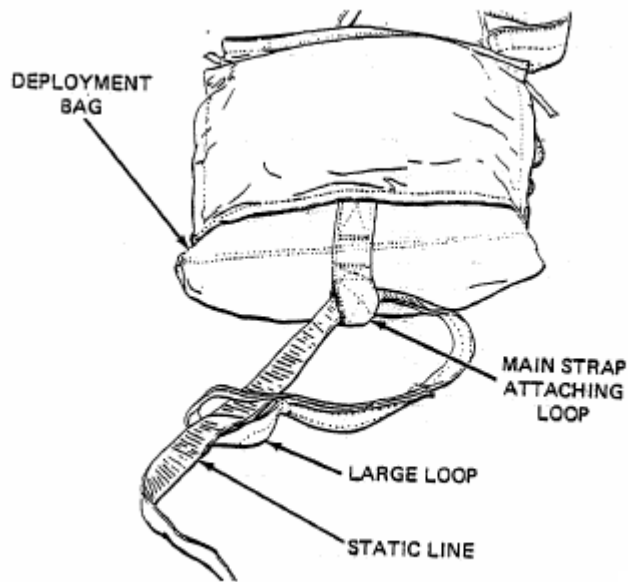
Figure 9. Attaching Static Line to Deployment Bag.
