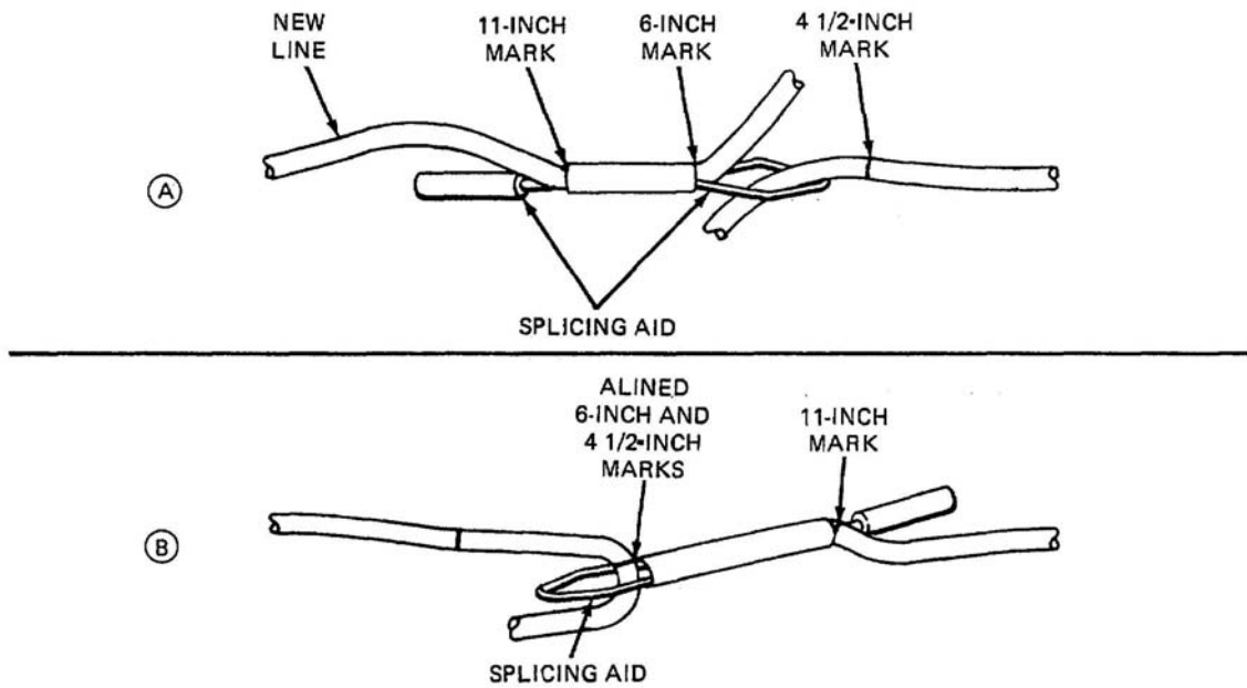
Figure 2. Inserting Splicing Aid into Cord Casing.
