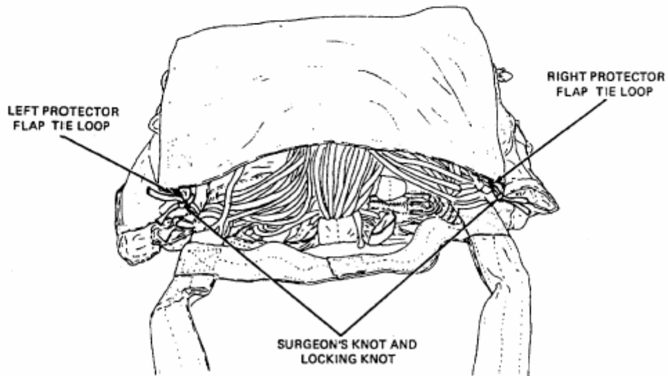
Figure 28. Suspension Line Protector Flap Closed and Secured.
