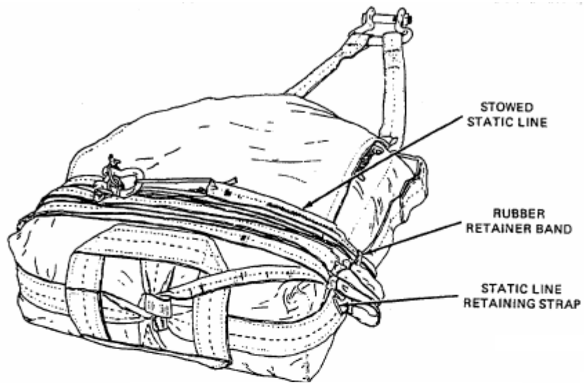
Figure 29. Static Line Stowed and Secured.
