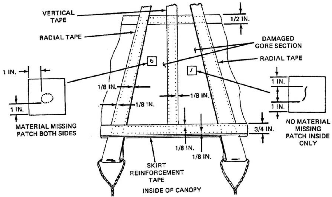
Figure 2. Pressure Sensitive Patch.
