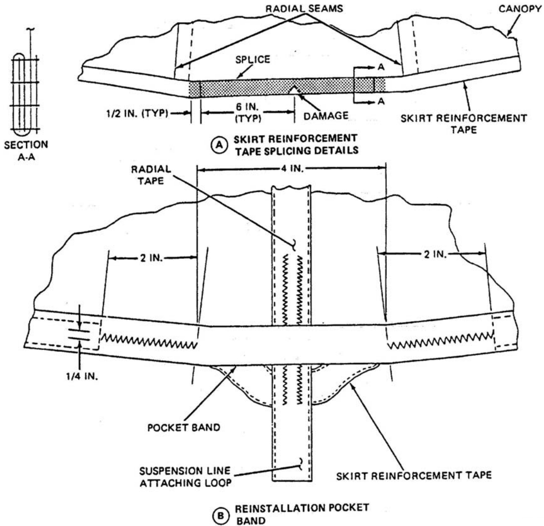
Figure 1. Skirt Reinforcement Tape Splicing Details.
