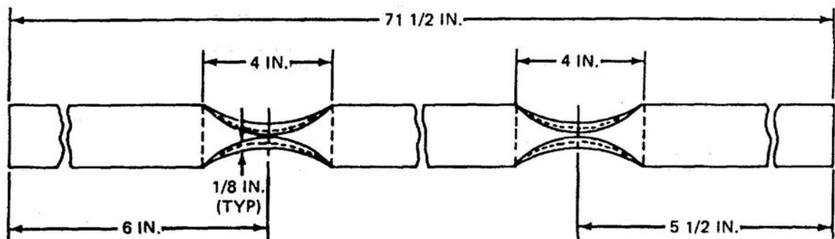
Figure 3. Riser Suspension Line Attaching Loops Construction Details.
