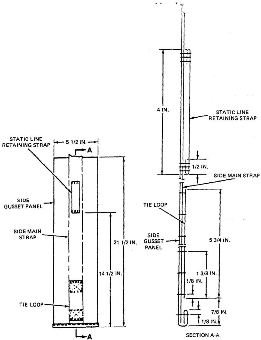
Figure 4. Side Main Strap Replacement Details.
