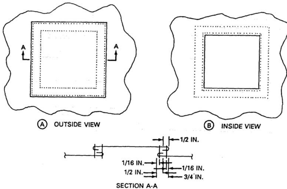
Figure 1. Patching Deployment Bag Panels and Flaps.
