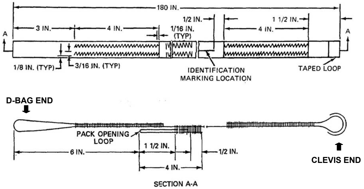
Figure 2. Static Line Construction Details.
