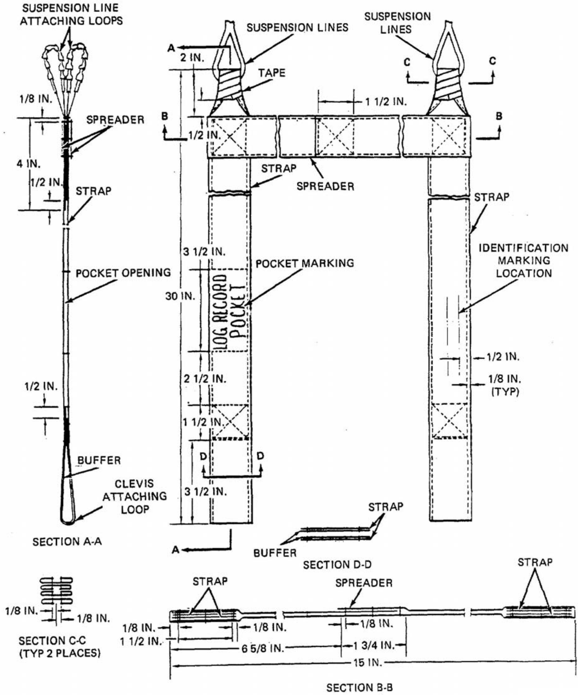
Figure 4. Riser Assembly Construction Details.
