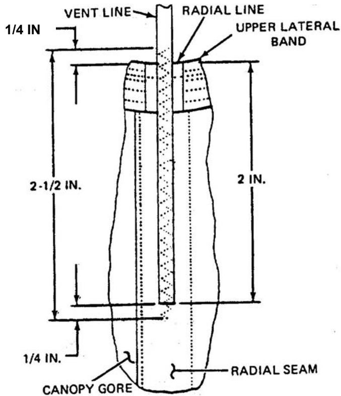
Figure 1. Vent Line Replacement Details.
