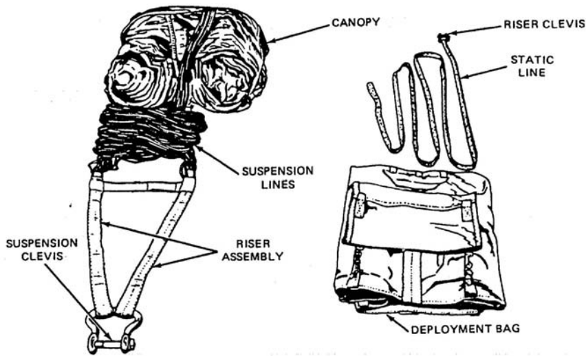
Figure 1. The 26-Foot Diameter, High-Velocity Cargo Parachute, with Deployment Bag.
