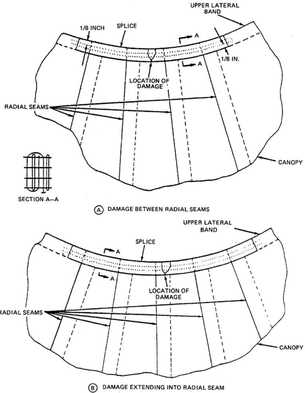
Figure 1. Vent Reinforcement Tape Splicing Details.
