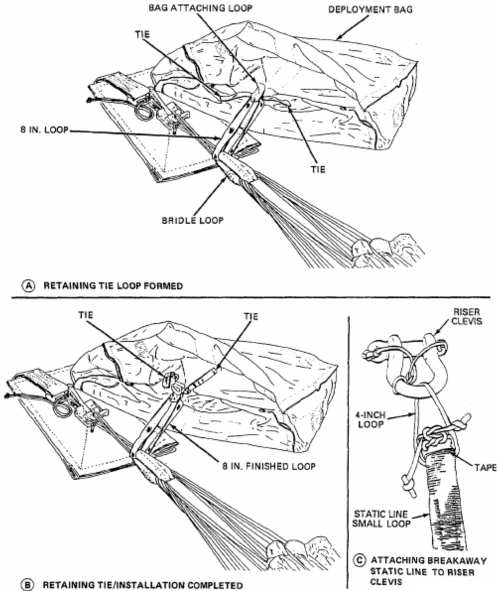
Figure 17. Attaching Cotton Deployment Bag Retaining Tie and Breakaway Static Lines.
