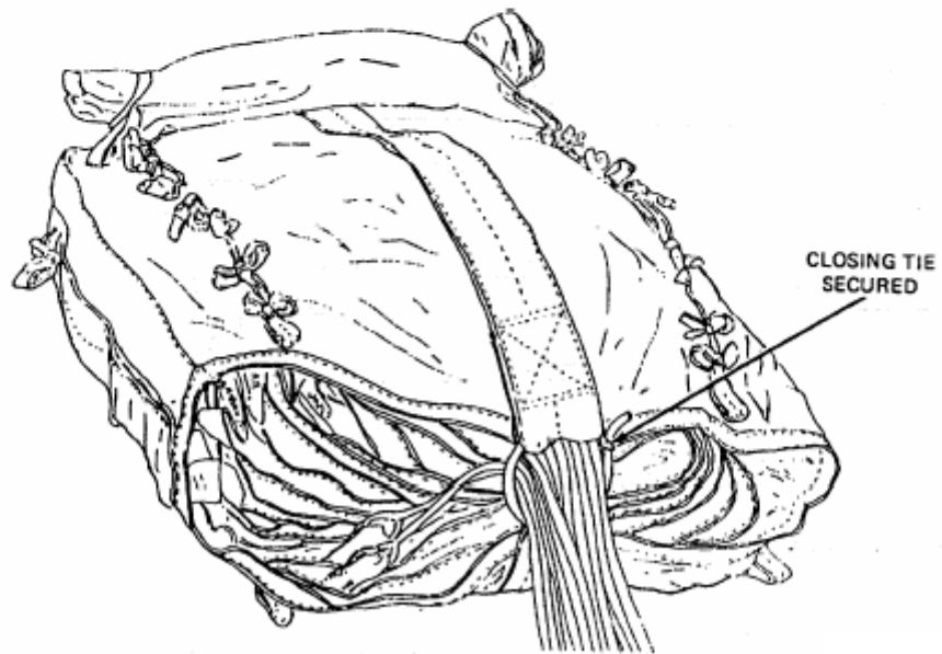
Figure 22. Bag Closing Tie Completed.
