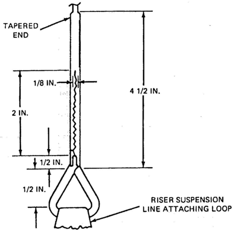
Figure 5. Securing Suspension Line at Riser Suspension Line Attaching Loop.
