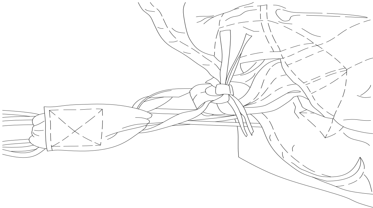
Figure 18. Attaching Nylon Bag for Non-Breakaway Static Line.
