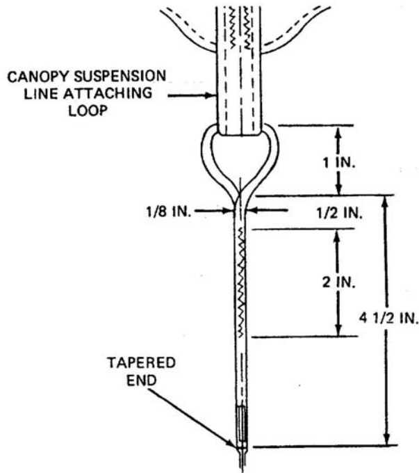
Figure 3. Securing Suspension Line at Suspension Line Attaching Loop.
