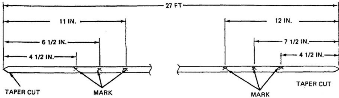
Figure 1. Replacement Suspension Line Construction Details.
