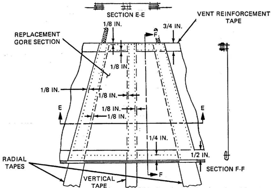
Figure 6. Gore Section 3, Replacement Details.
