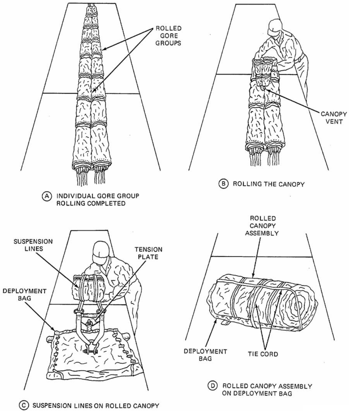
Figure 2, A-D. Rigger Rolling a Parachute Canopy Assembly.
