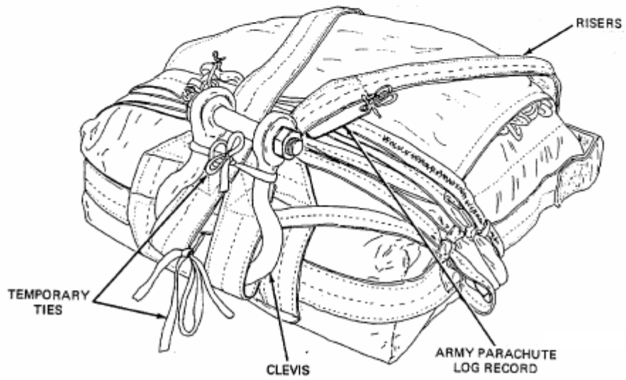
Figure 30. Parachute Pack Completed.
